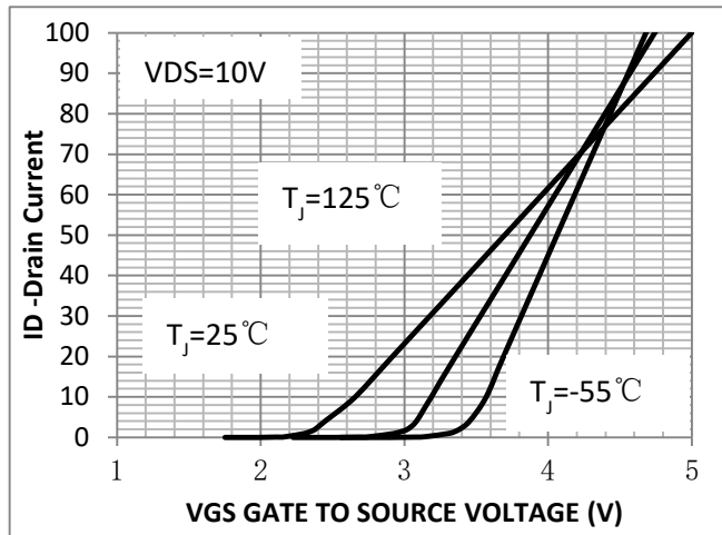
Figure 10. Transfer Characteristics
