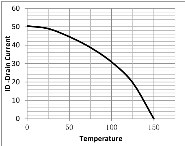
Fig.8 ID-Junction Temperature
